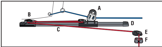
Barbarhauler: Use this low-profile system on racing boats with nonoverlapping jibs like the Farr® 40 and One Design 35. An inhaul is used to control slot size.
