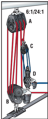
6:1/24:1 Cascaded: This 6:1/24:1 system is used on boats with mains as large as 25.5 m² (275 ft²) and end-boom sheeting.
