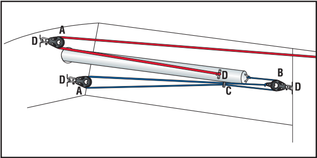
Pole Launcher: Many racing boats have asymmetrical spinnakers and retractable bowsprits. This system features a launcher line on top of the pole, with strong shockcord on the bottom to automatically retract the pole when the launcher line is uncleated.
