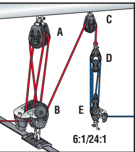
6:1/24:1 Gross/Fine: This 6:1/24:1 cascading system is used on boats with end-boom sheeting and mains as large as 25.5 m² (275 ft²) and end-boom sheeting.
