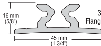
2720 Small Boat traveler track
