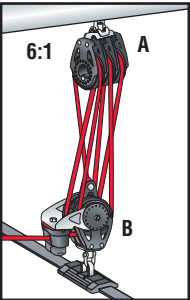
6:1 Reeved Right Angle: Boats with mainsails to 35 m² (375 ft²) often use a 6:1 system.
